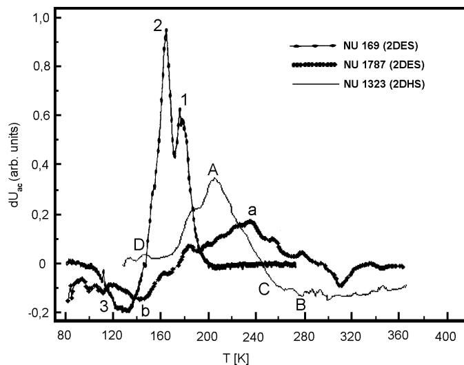
Fig. 3. A-DLTS spectra of investigated GaAs/AlGaAs heterostructures obtained for a relaxation time \tau = 0.0368 s.
