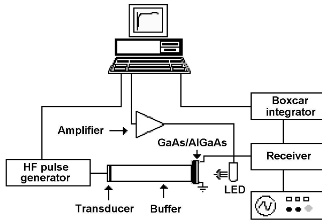
Fig. 1. The experimental setup to perform acoustoelectric response signal versus temperature measured under (after) illumination.
